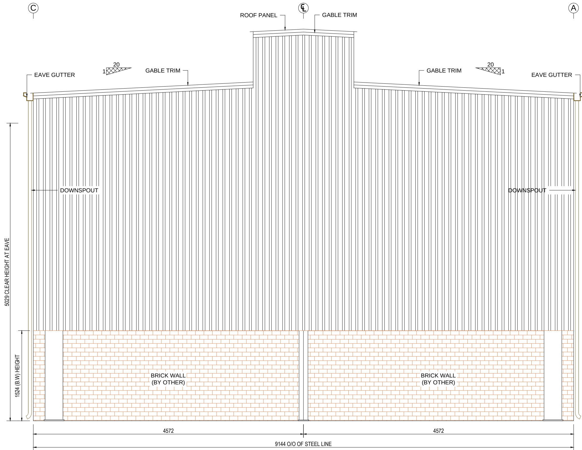
END WALL SHEETING @ GRID-3
